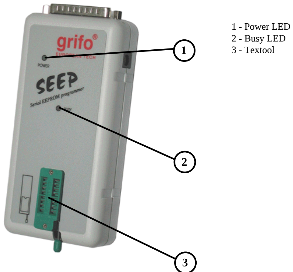
FIGURE 5: LEDs AND TEXTTOOL LOCATION
